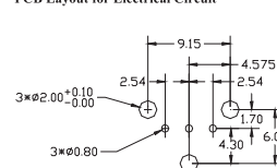
PCB Layout for Electrical Circuit
