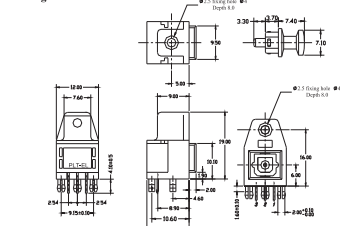
Package Dimensions
