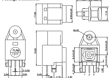
Package Dimensions
