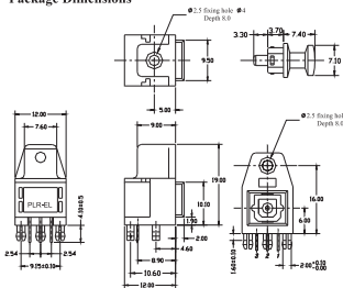
Package Dimensions
