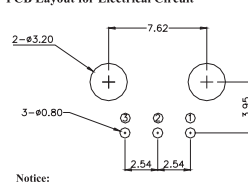
PCB Layout for Electrical Circuit
