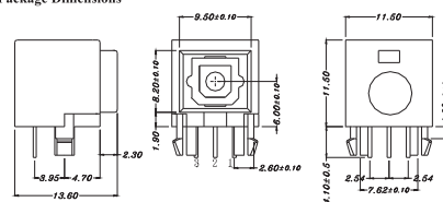
Package Dimensions
