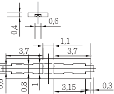
Soldering patterns
