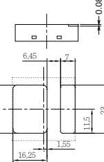
Soldering patterns
