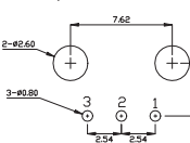
PCB Layout for Electrical Circuit
