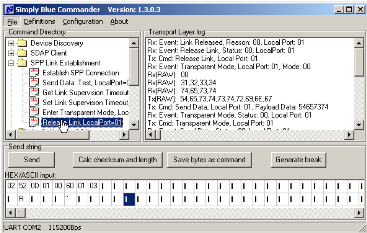
Figure 2-47. Releasing the link by the LMX9820A/LMX9830/LMX9838
