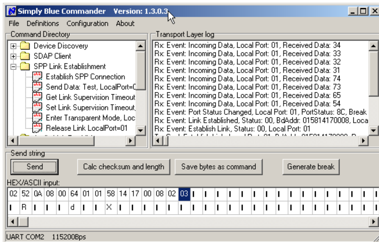
Figure 2-38. Incoming Data at LMX9820A/LMX9830/LMX9838 in command mode
