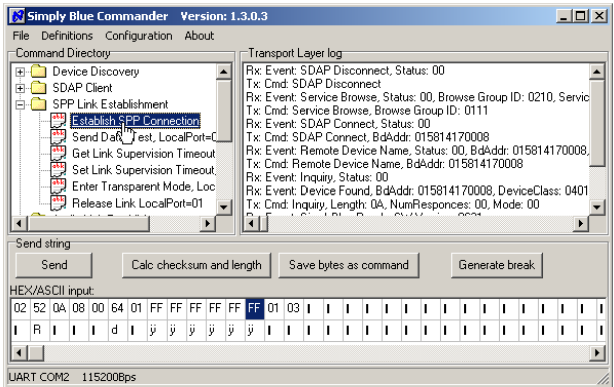
Figure 2-29. Select “Establish SPP Link”
