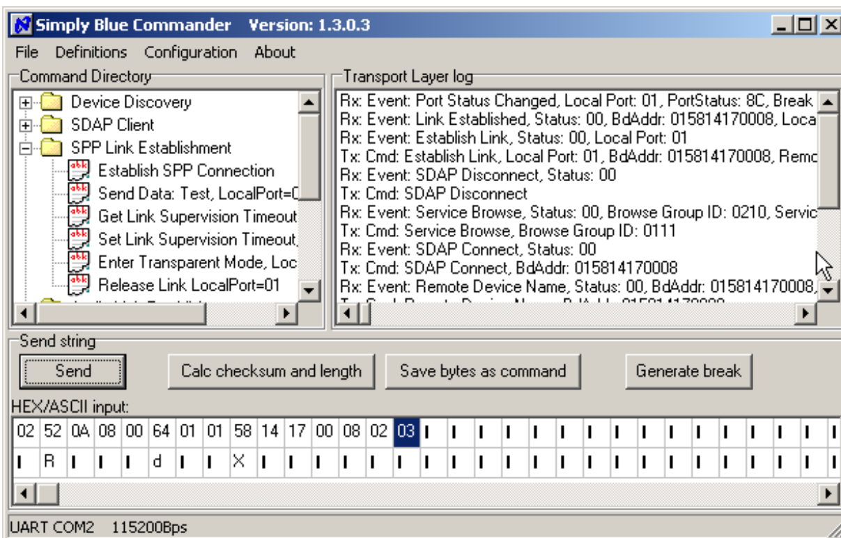
Figure 2-34. Successful link establishment from the LMX9820A/LMX9830/LMX9838
