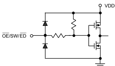
\overline{OE}/SW/\overline{ED} Terminal
