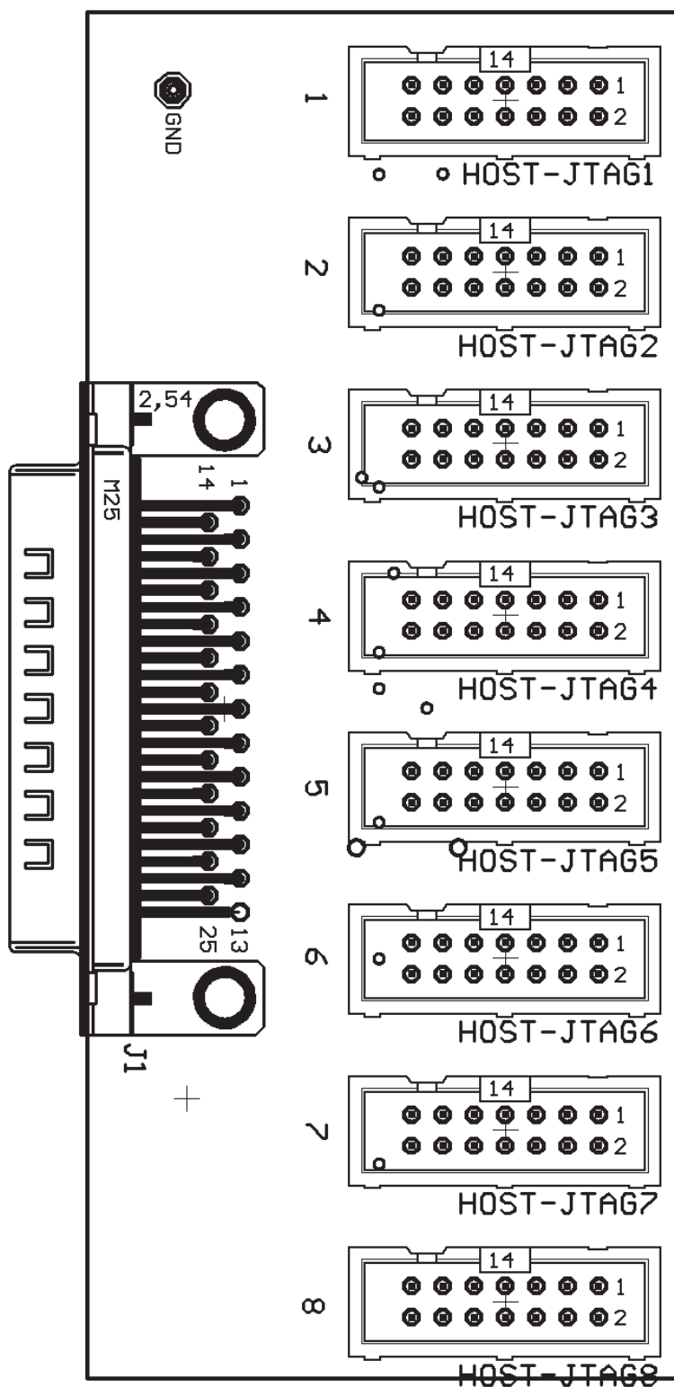
Figure 5-6. Gang_Exp Layout
