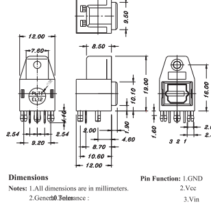
Package
