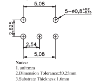
PCB Layout for Electrical Circuit
