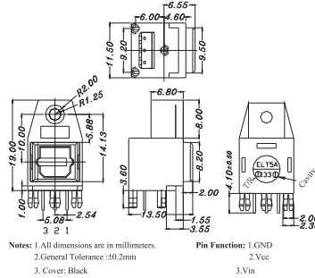
Package Dimensions
