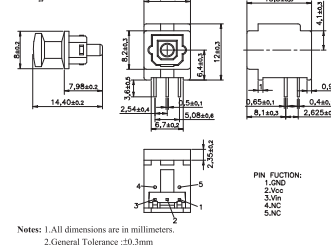
Package Dimensions
