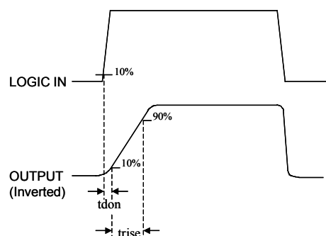
Switching Waveforms
