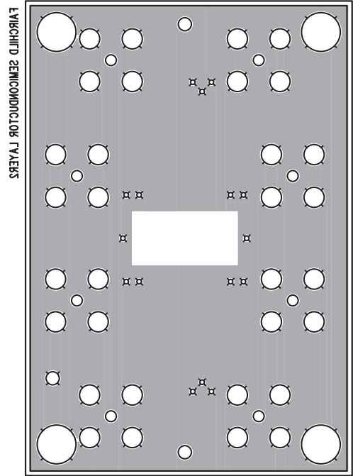
Figure 43. FHP3450 KEB018 (bottom side)
