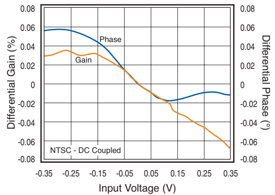
Figure 24. Differential Gain and Phase ( \pm 2.5\text{V} )
