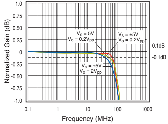
Figure 8. Gain Flatness vs. Frequency
