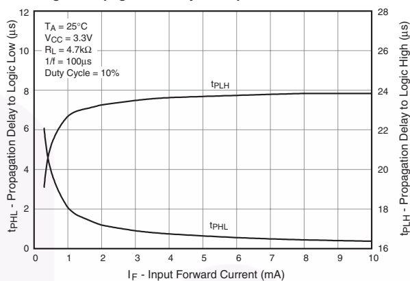
Fig. 8 Propagation Delay vs. Input Forward Current
