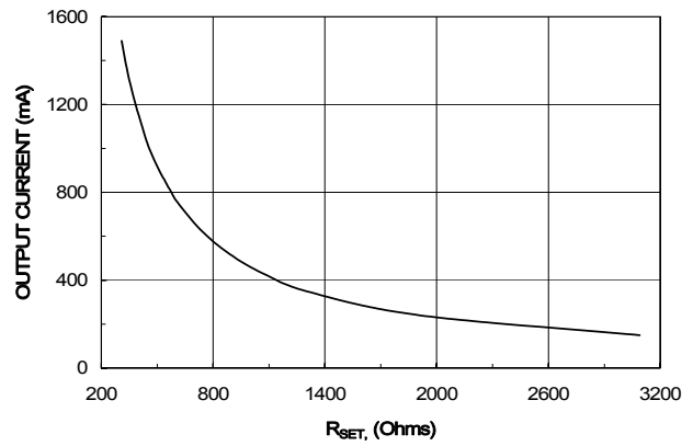
Figure 10. Current Limit vs. Rest
