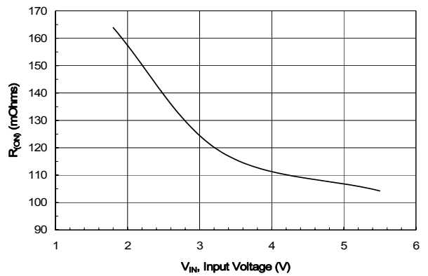
Figure 12. R_{ON} vs. V_{IN}
