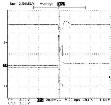
Figure 22. Short Circuit Response (Output Shorted to GND)
