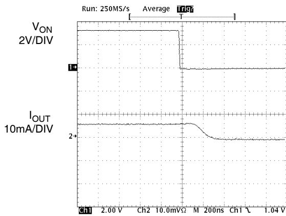
Figure 21. T_{OFF} Response
