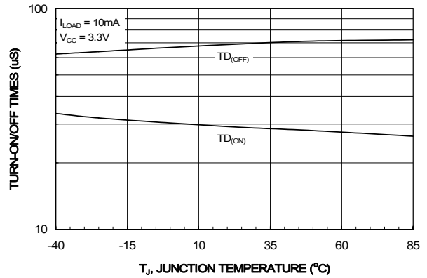
Figure 14. T_{ON}/T_{OFF} vs. Temperature
