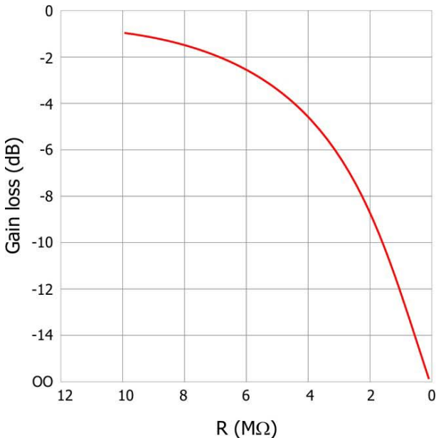
Fig. 2 Attenuation curve according to RX value
