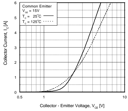
Fig 2. Typical Saturation Voltage Characteristics
