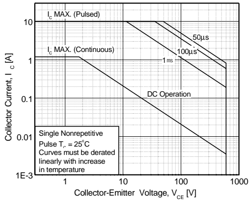
Fig 15. SOA Characteristics
