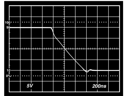
TPC 24. Negative Slew Rate R_L = 2\text{ k}\Omega , V_S = \pm 15\text{ V} , A_V = +1
