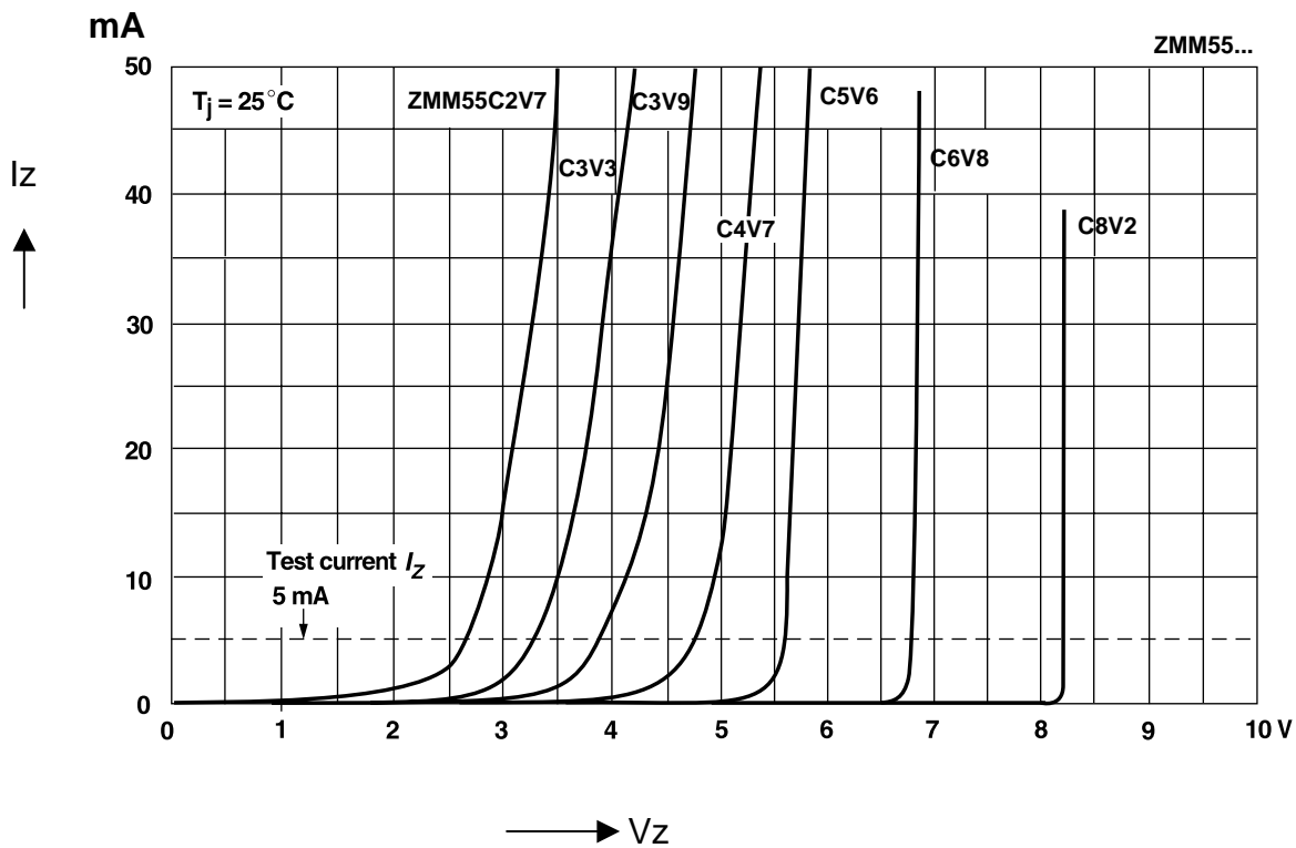
FIG.1- BREAKDOWN CHARACTERISTICS
