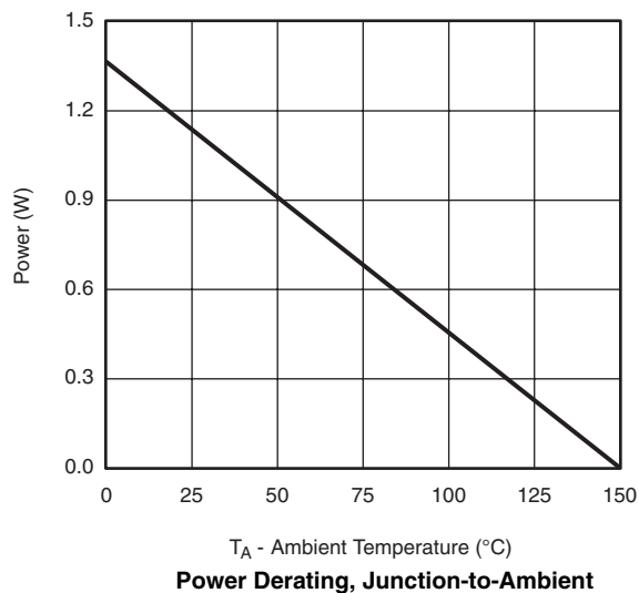
Power Derating, Junction-to-Ambient
