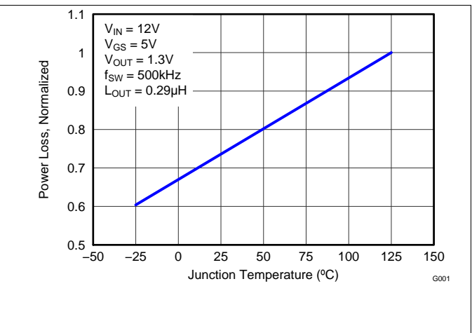
Figure 2. Normalized Power Loss vs Temperature
