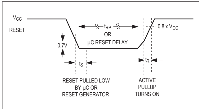
Figure 5. Bidirectional RESET Timing Diagram
