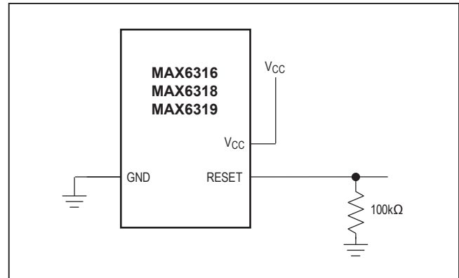
Figure 8. Ensuring RESET Valid to V_{CC} = 0V on Active-Low Push/Pull and Bidirectional Outputs
