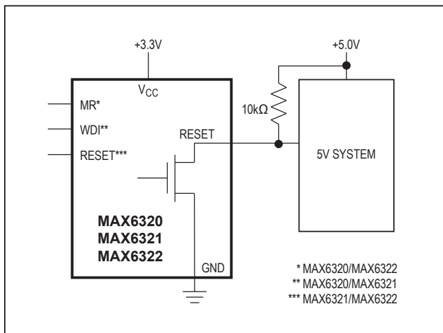
Figure 6. MAX6320P/MAX6321HP/MAX6322HP Open-Drain RESET Output Allows Use with Multiple Supplies
