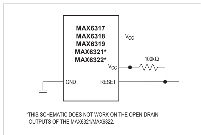
Figure 9. Ensuring RESET Valid to V_{CC} = 0V on Active-High Push/Pull Outputs
