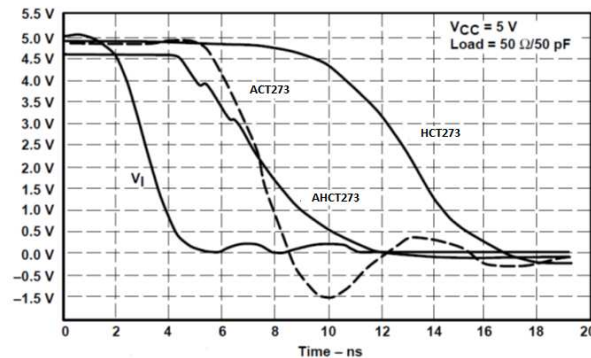
Figure 6. Switching Characteristics Comparison
