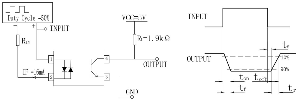
图 2 t_{\text{on}}, t_s, t_{\text{off}} 测试方法 Figure 2- The test method of t_{\text{on}}, t_s, t_{\text{off}}
