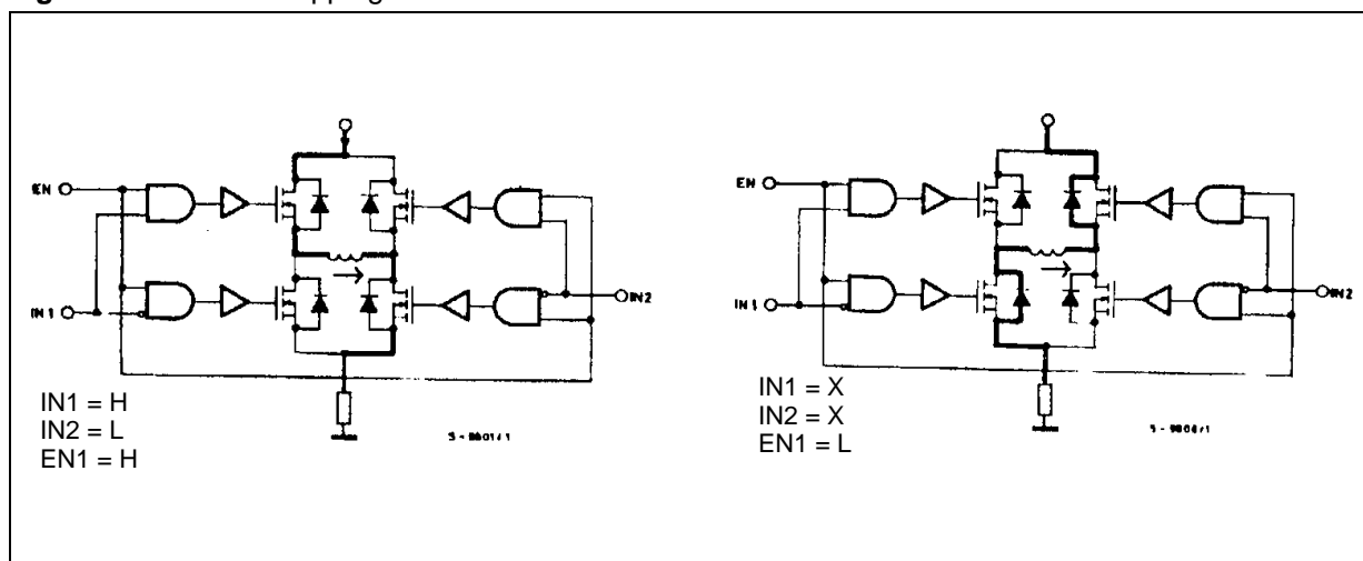
Figure 3c: Enable Chopping
