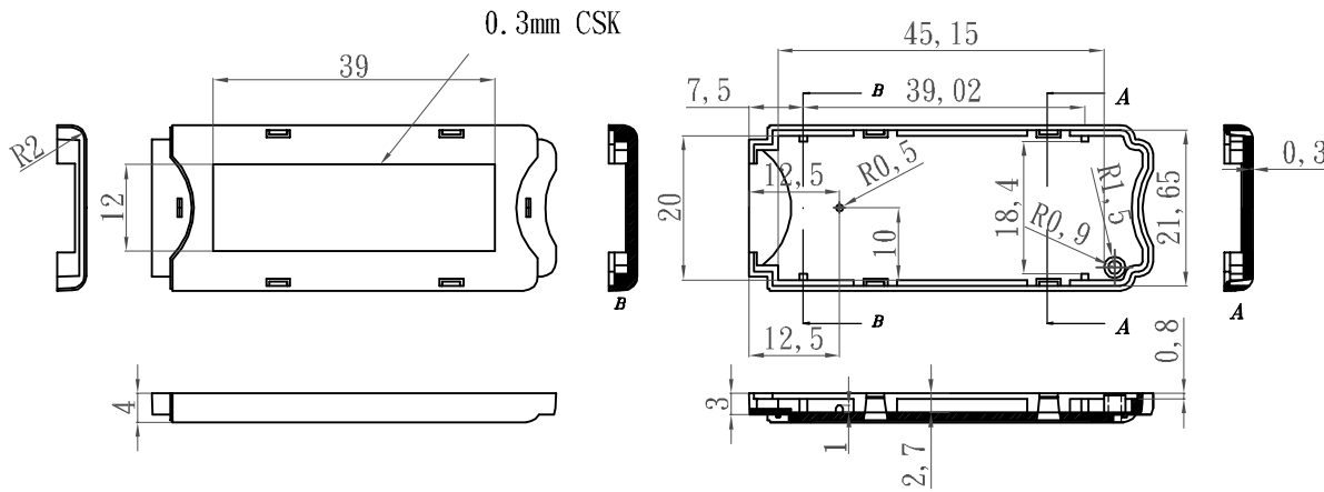
BASE
