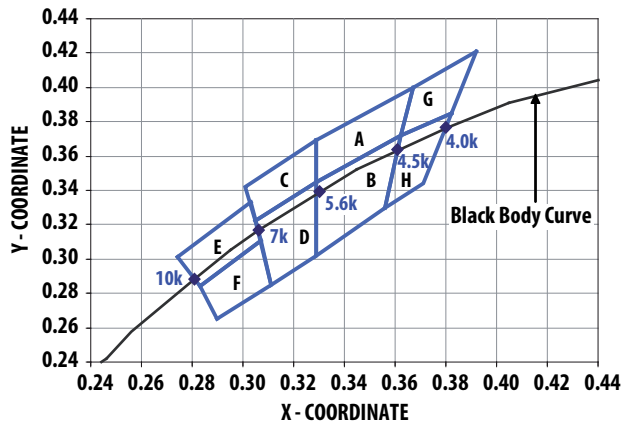
Figure 15. Color bins (Cool White).
