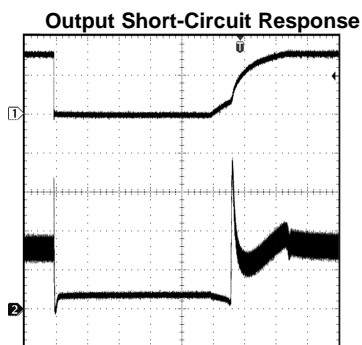
V_{IN} = 3.6V , I_{LED} = 30mA Channel 1: V_{OUT} (10V/div) Channel 2: I_{IN} (100mA/div) Time Base: 200µs/div
