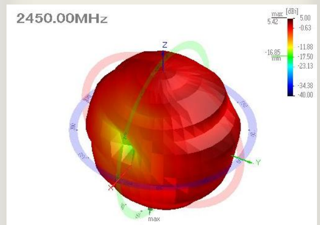
[3D Radiation Pattern]
