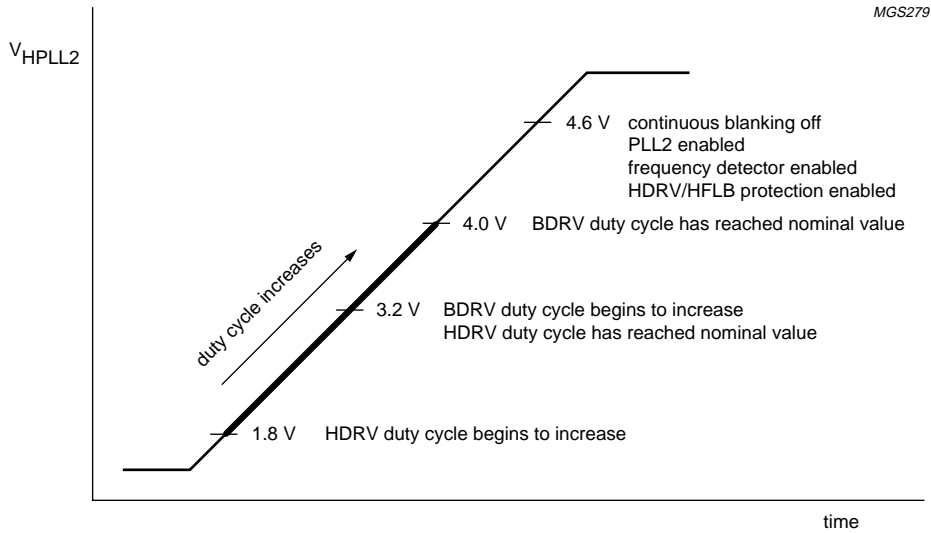
a. PLL2 soft start sequence, if V_{CC} > 8.6 V.
