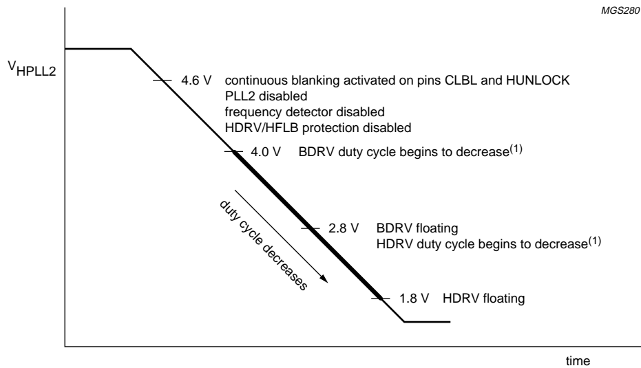
b. PLL2 soft-down sequence, if V_{CC} > 8.6 V.
