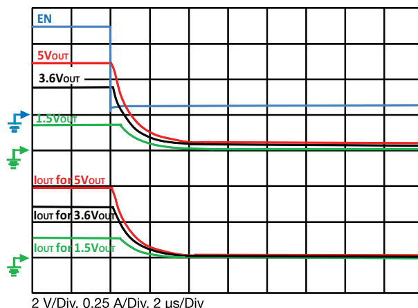
Fig. 22 - Typical Fall Time C OUT = 0.1 μF, C IN = 4.7 μF, R OUT = 10 Ω
