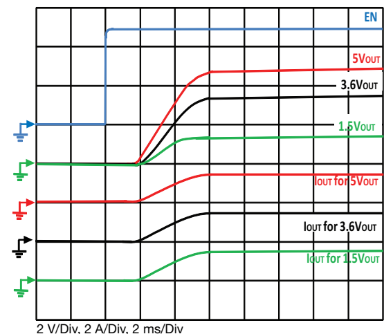
Fig. 20 - Typical Turn-on Delay, Rise Time C OUT = 200 μF, C IN = 4.7 μF, I OUT = 1.5 A
