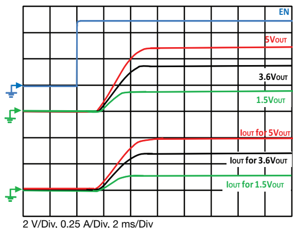
Fig. 19 - Typical Turn-on Delay, Rise Time C OUT = 0.1 μF, C IN = 4.7 μF, R OUT = 10 Ω
