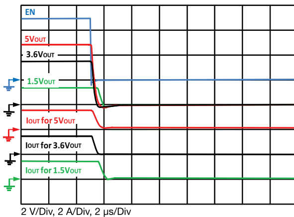
Fig. 21 - Typical Fall Time C OUT = 0.1 μF, C IN = 4.7 μF, I OUT = 1.5 A
