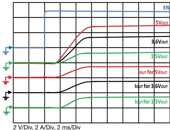
Fig. 18 - Typical Turn-on Delay, Rise Time C OUT = 0.1 μF, C IN = 4.7 μF, I OUT = 1.5 A
