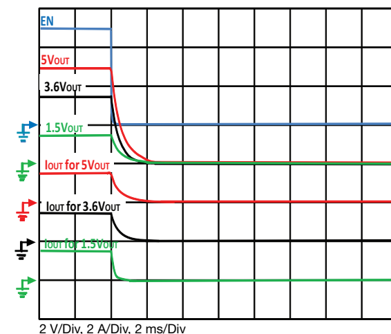
Fig. 23 - Typical Fall Time C OUT = 200 μF, C IN = 4.7 μF, I OUT = 1.5 A
