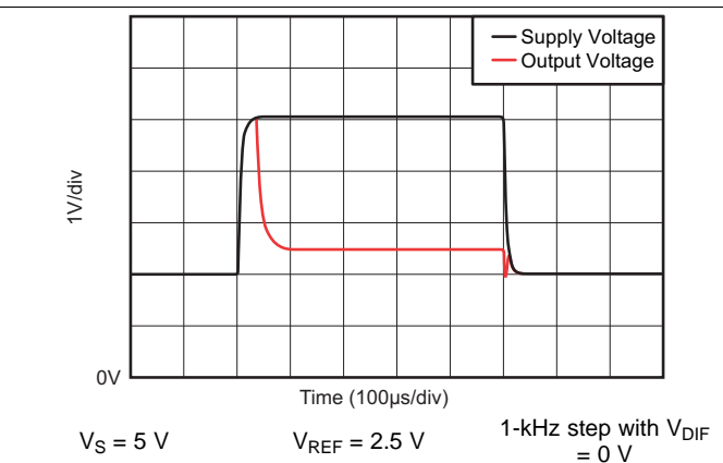
Figure 22. Brownout Recovery
