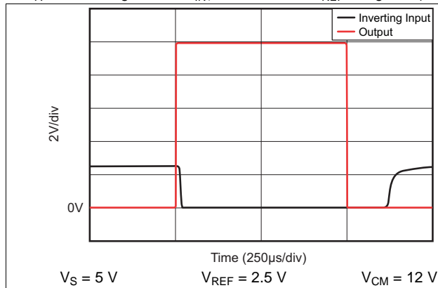
Figure 19. Inverting Differential Input Overload
