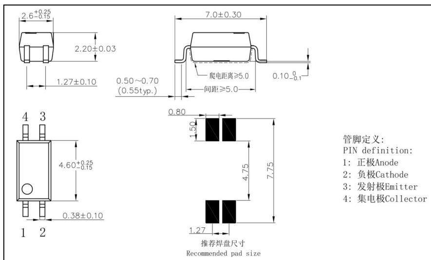
图 4 HPC217S-(R) 外形尺寸 Figure 4- The dimensions of HPC217S-(R)
