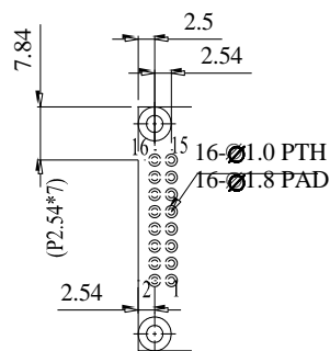
PIN DETAIL
