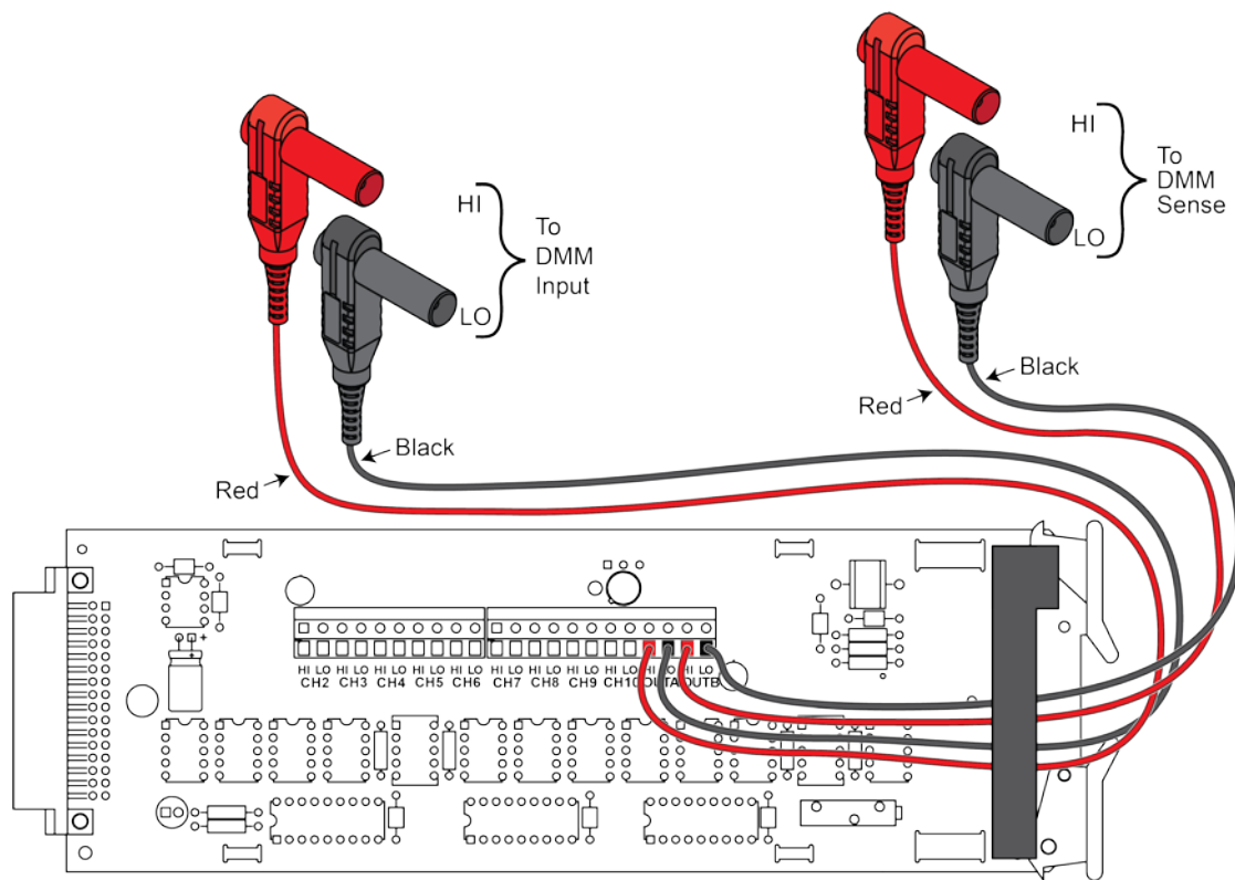
Figure 37: 2001-TCSCAN card
