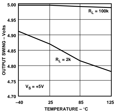
Figure 26. Output Voltage Swing vs. Temperature, V_S = +5 V
