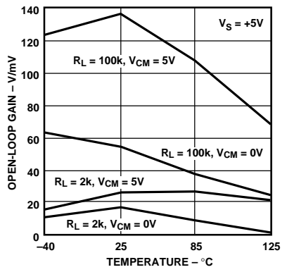
Figure 28. Open-Loop Gain vs. Temperature, V_S = +5 V
