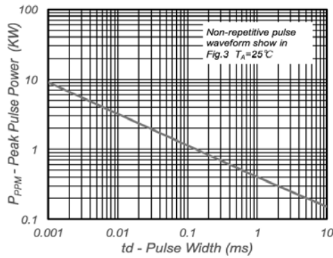
Fig.1 Peak Pulse Power Rating
