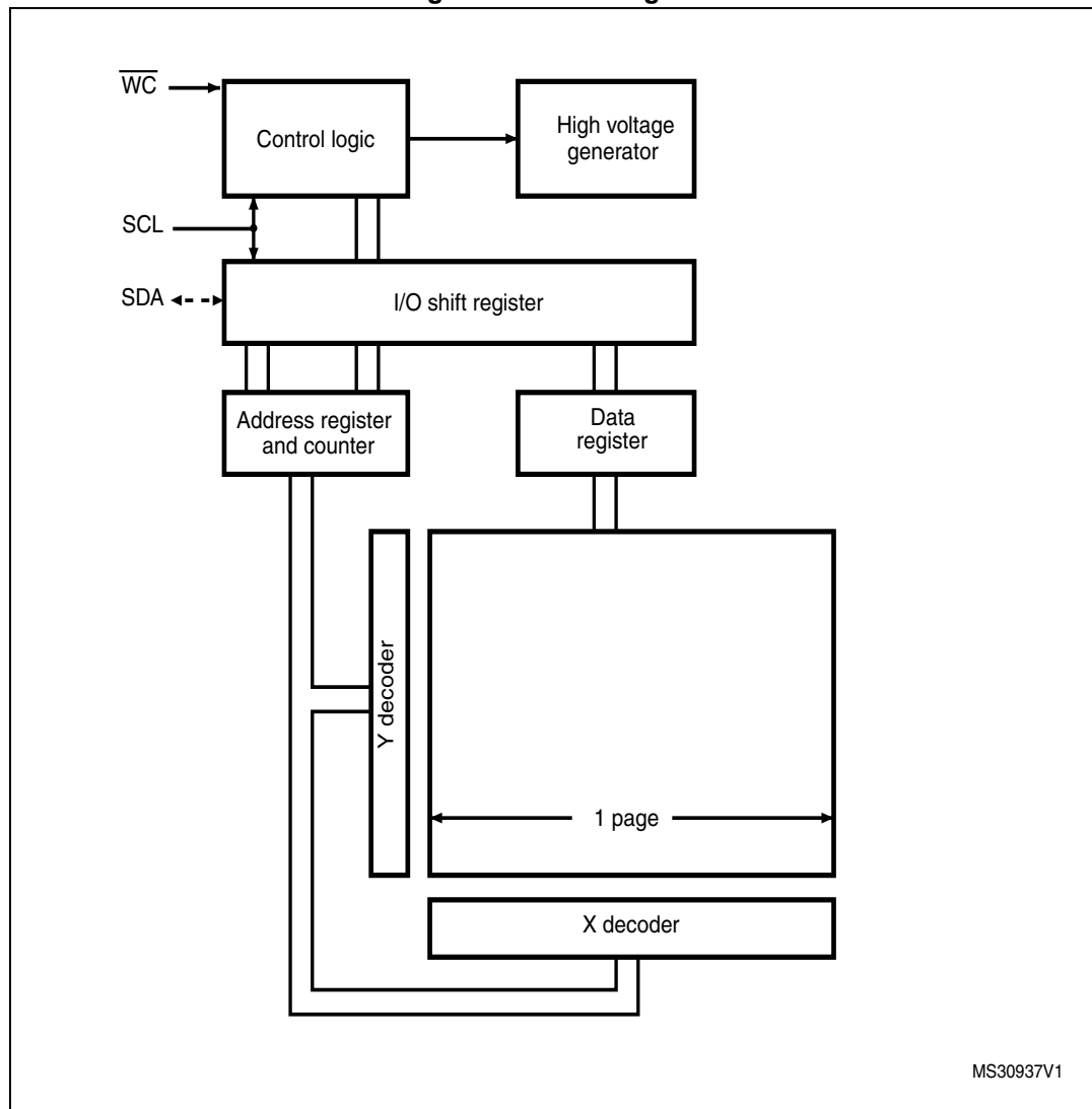
Figure 5. Block diagram
