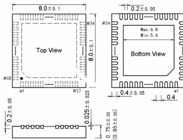
Figure 5-2 QFN68X8 package
