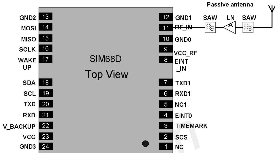
Figure 8: SIM68D passive antenna design for best performance and increased immunity
