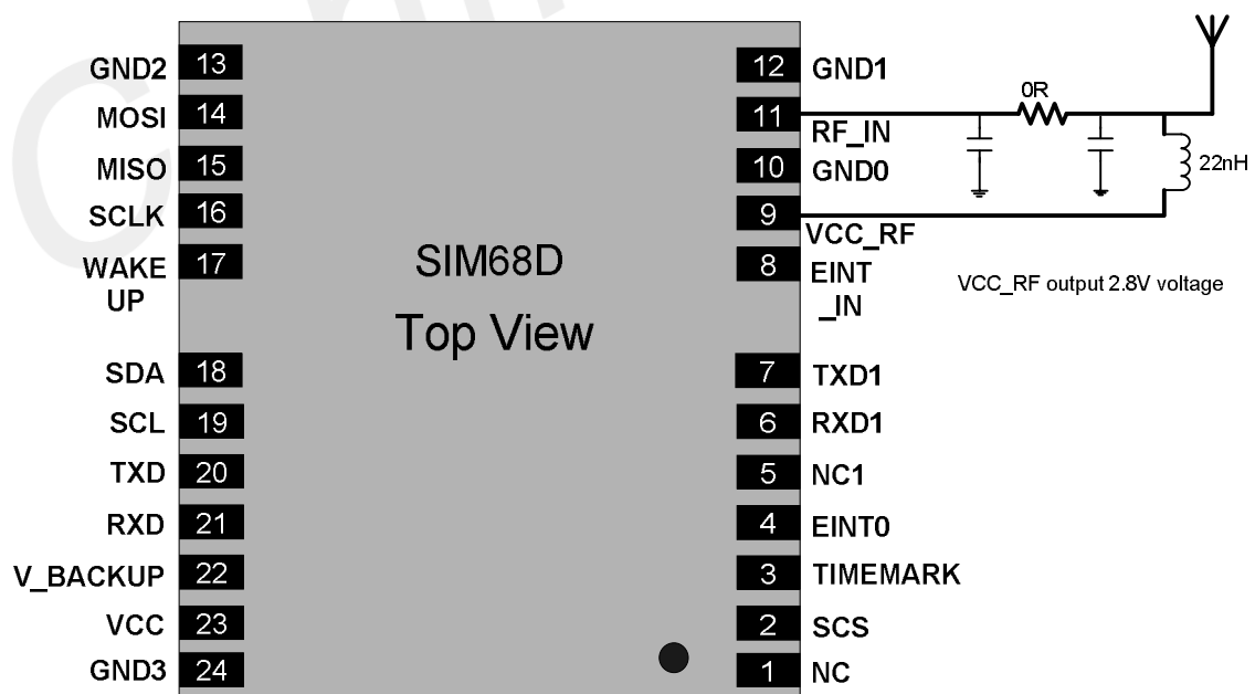
Figure 9: SIM68D active antenna design
