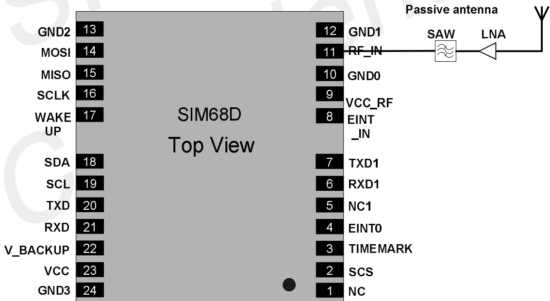
Figure 7: SIM68D passive antenna design (with external LNA and SAW)
