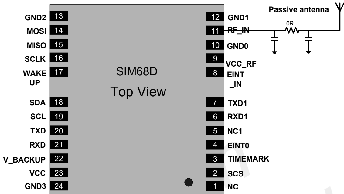
Figure 6: SIM68D passive antenna design
