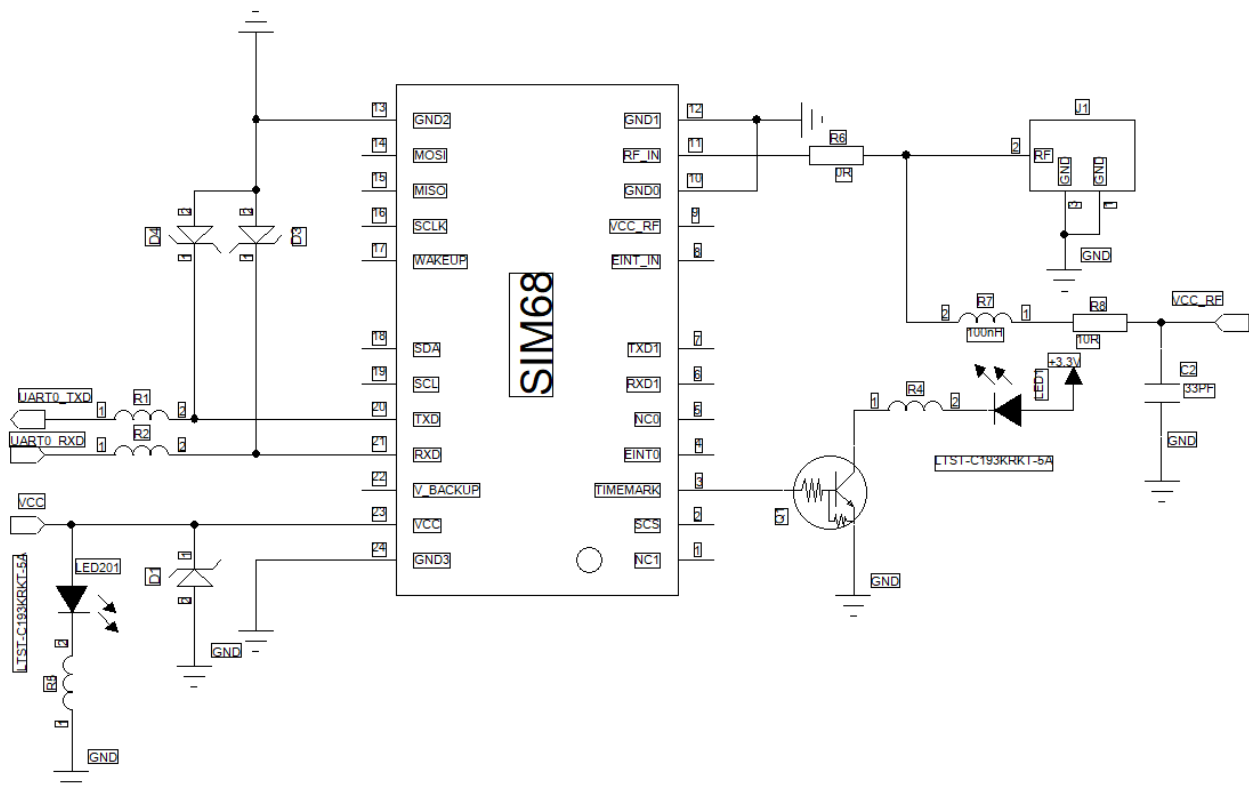
Figure 13: Example application schematic
