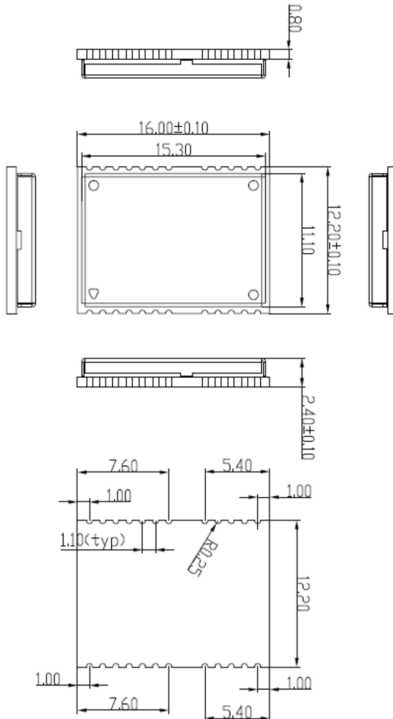
Figure 3: SIM68D mechanical dimensions (Unit: mm)
