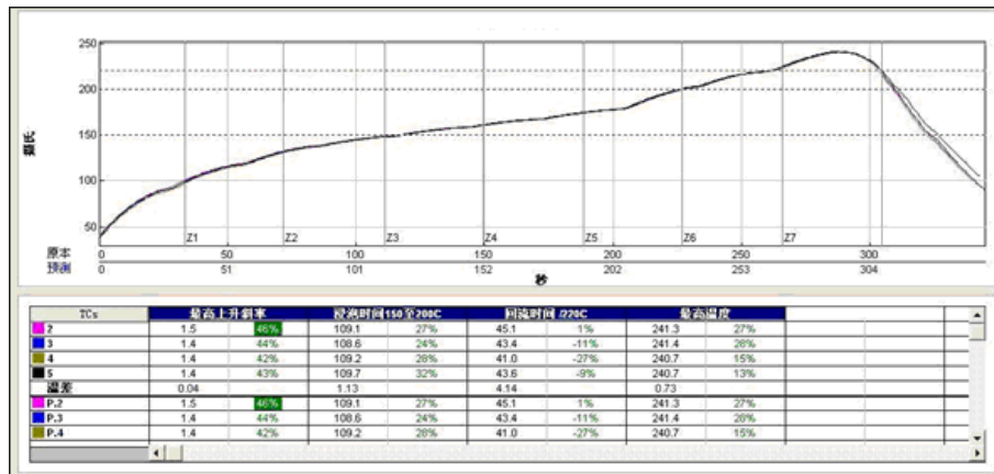
Figure 12: The Ramp-Soak-Spike reflow profile of SIM68D
