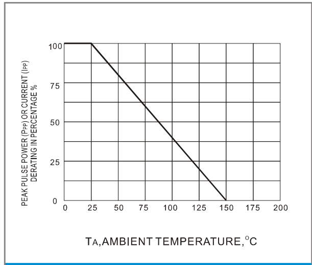
Fig.2 DERATING CURVE
