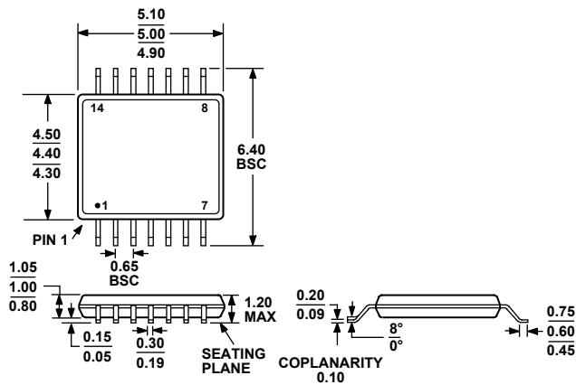
COMPLIANT TO JEDEC STANDARDS MO-153-AB-1 Figure 29. 14-Lead Thin Shrink Small Outline Package [TSSOP] (RU-14) Dimensions shown in millimeters
