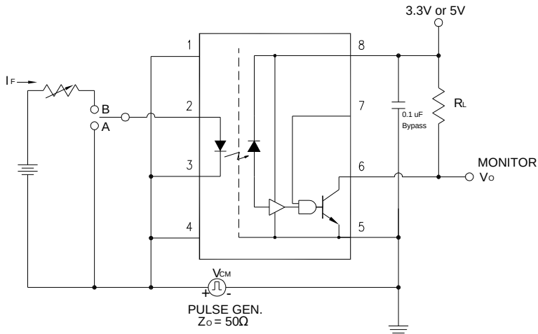
Figure 3: Single Channel Test Circuit for Common Mode Transient Immunity
