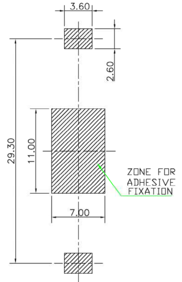
PCB LAYOUT
