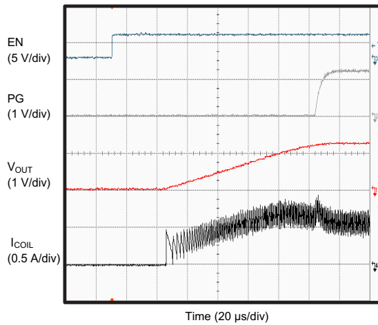
V_{IN} = 3.3\text{ V} , V_{OUT} = 1.2\text{ V} , Load = 2.2 Ω
