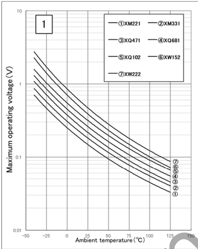
Graph of Maximum Operating Voltage Reduction Characteristics
