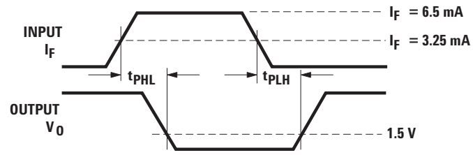
Figure 6. Test Circuit for t PHL and t PLH
