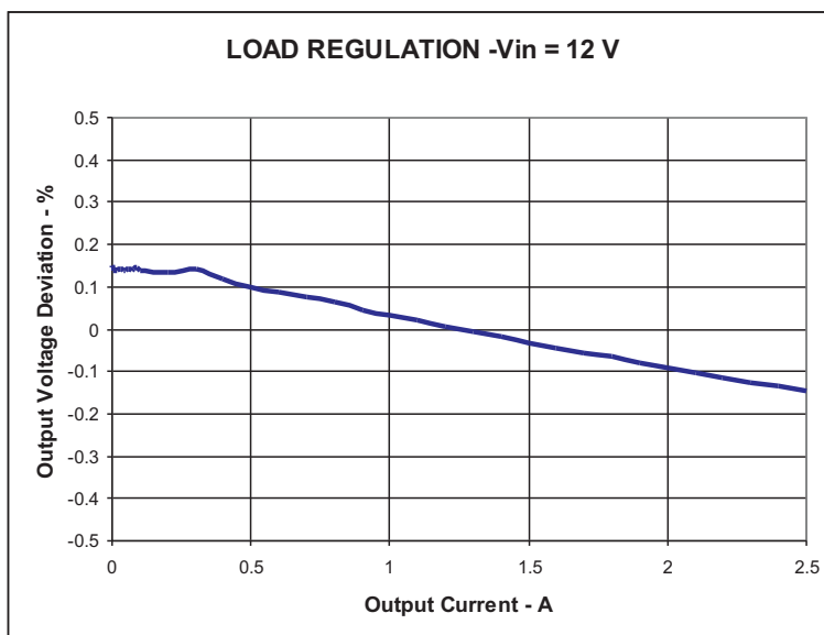
Figure 3. TPS54260EVM-597 Load Regulation
