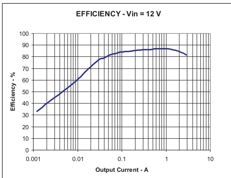
Figure 2. TPS54260EVM-597 Low Current Efficiency
