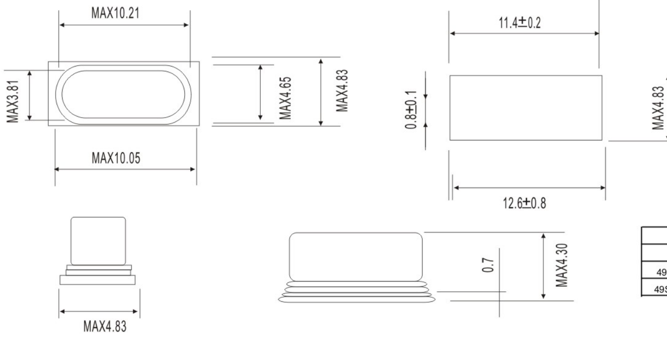
49S-SMD/49S2-SMD
