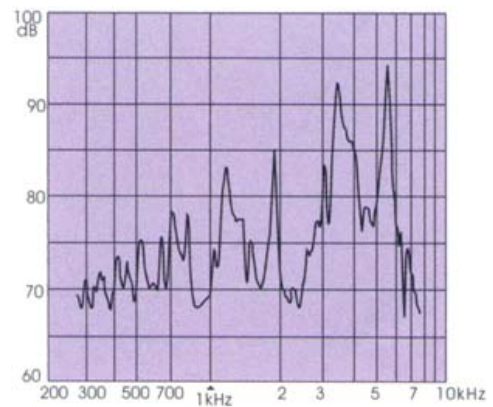
TFM-35 3V P-P Square Wave /10cm
