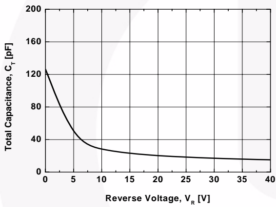
Figure 3. Total Capacitance
