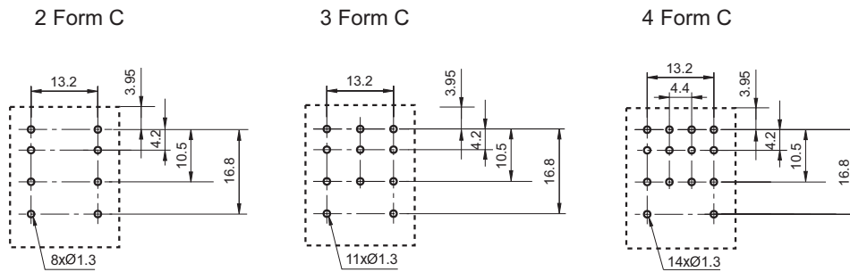
Wiring Diagram (Bottom view)
