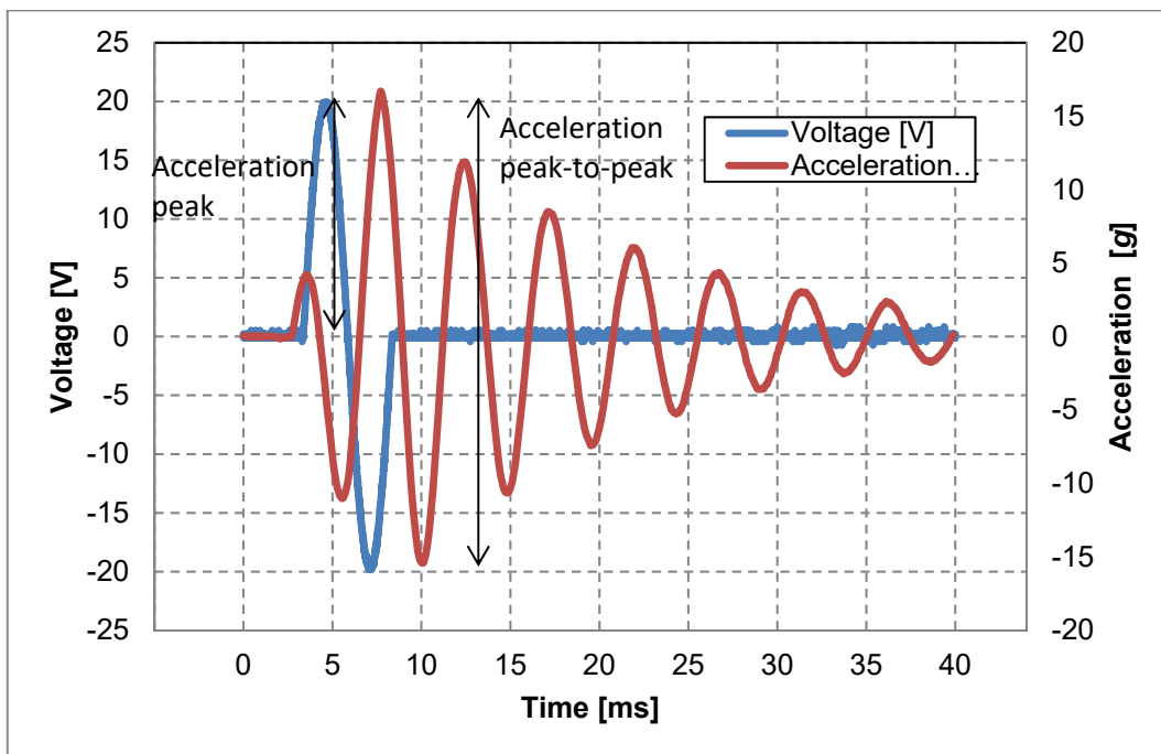
Fig. 6: Typical acceleration g as a function of input voltage with 100 g load. Input voltage with a sinus signal form of amplitude -20 \dots 20 V and pulse length 5 ms which is equivalent to 200 Hz.
