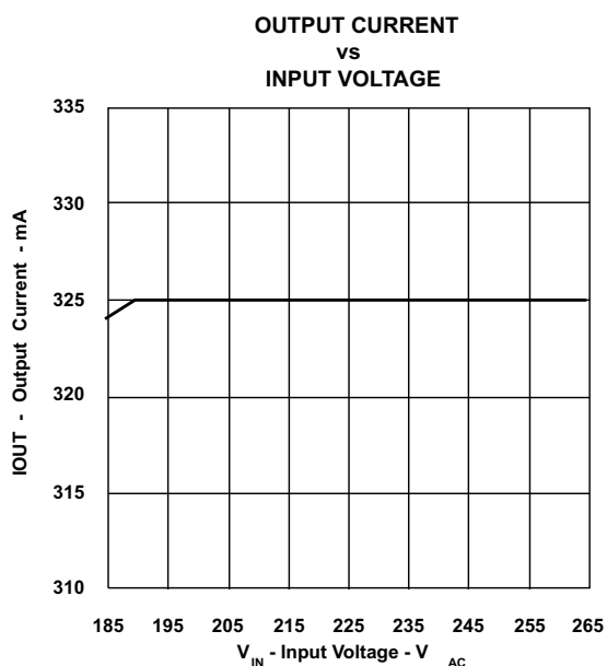
Figure 8. Line Regulation
