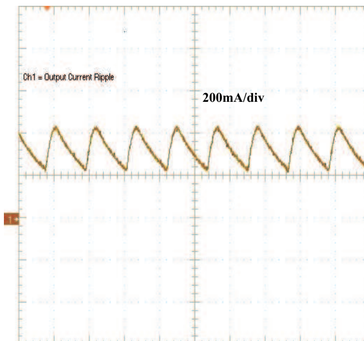
Figure 10. Output Current Ripple with Dimmer at 0% Dim, (10 µs/div.)
