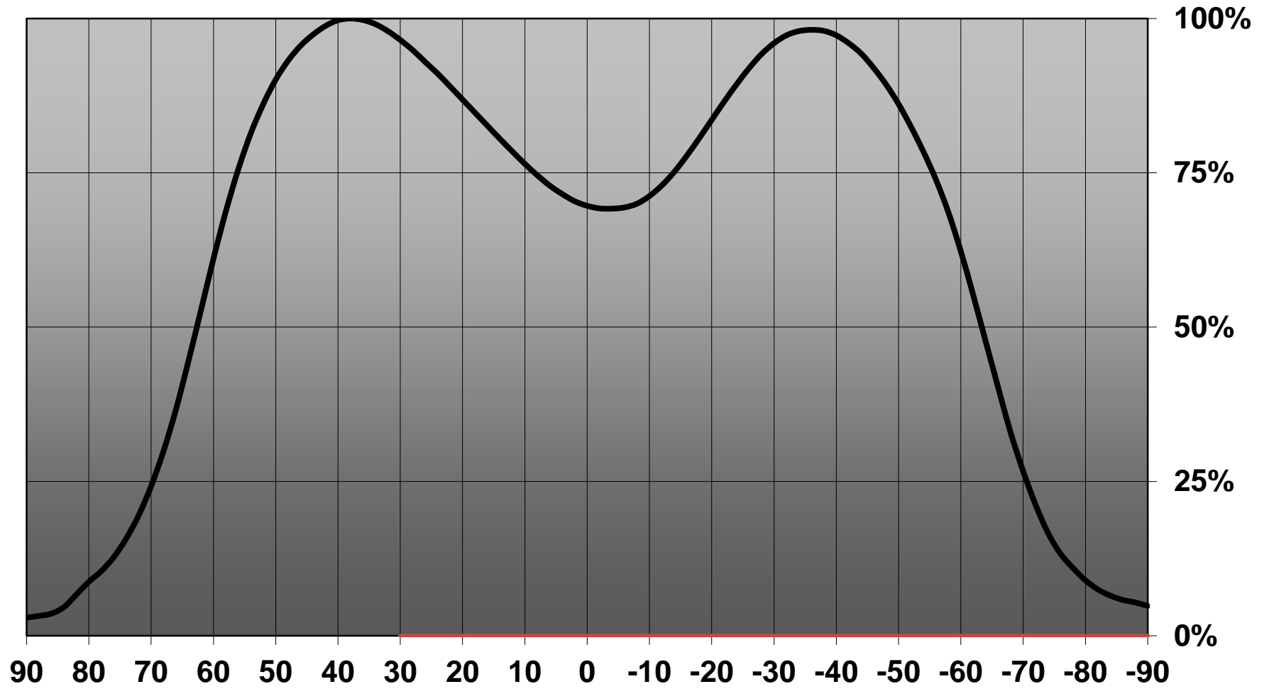
Relative intensity of CA11253_STRADA-C2-LuxR
