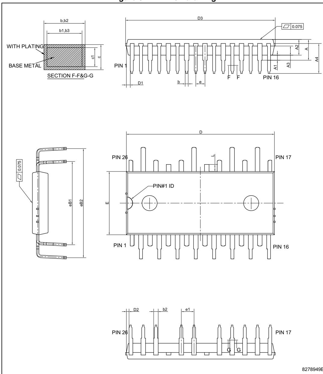
Figure 8. NDIP-26L drawing
